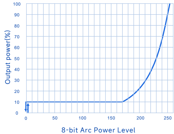
Logarithmic Dimming Curve:(DALI-2 Model)
