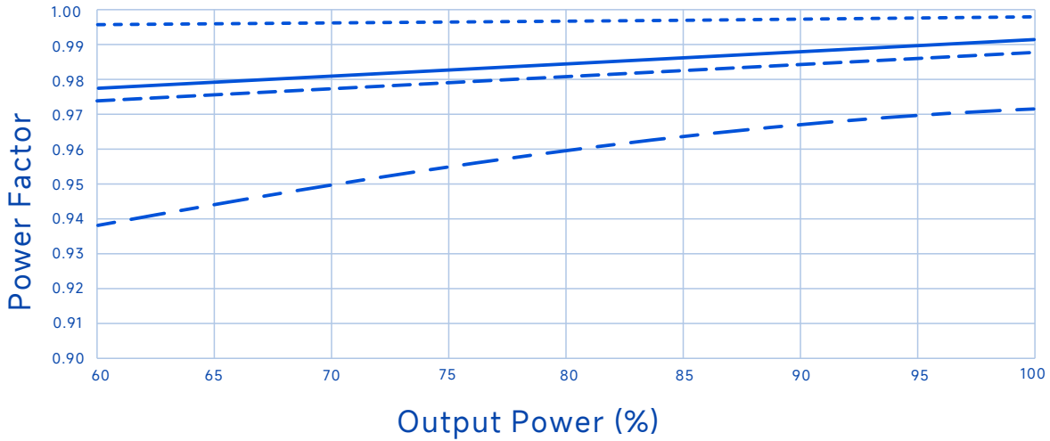
Power Factor Vs. O/P Power
