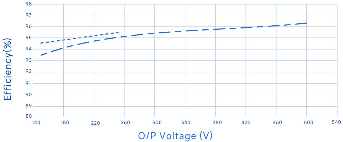
Efficiency Vs. O/P Voltage ( V_{in}=220V_{ac} )
